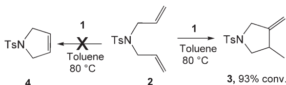
Scheme 3. Cycloisomerisation of diallyl- N -tosylamine.
