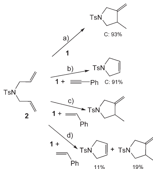
Scheme 4. RCM vs. cycloisomerisation. Reaction conditions: a) 5 mol % of 1 , toluene, 80 °C, 3 h. b) Same as a) + 10 mol % of phenylacetylene, toluene, 80 °C, 3 h. c) Same as a) + 25 mol % of styrene, toluene, 80 °C, 3 h. d) Same as a) + 25 mol % of styrene, 30 min at 90 °C before addition of 2 .
