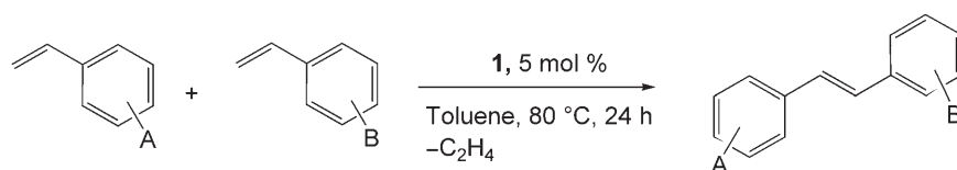
Scheme 2. Synthesis of unsymmetrical stilbenes.
