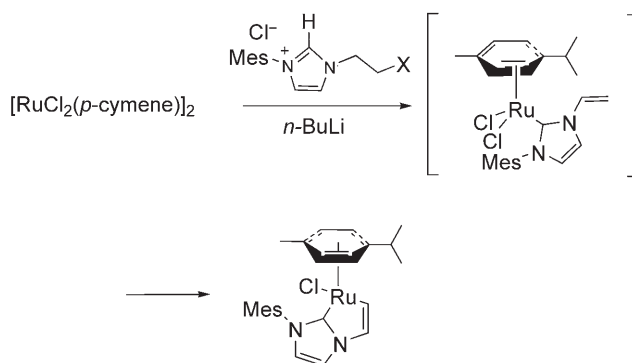
Scheme 1. Intramolecular vinyl C–H bond activation.
