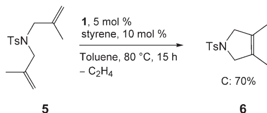
Scheme 5. RCM of a sterically hindered substrate.
